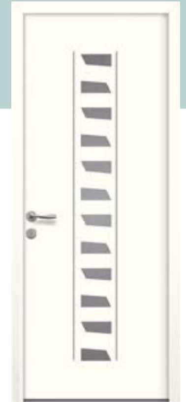
AURÉLIA €€€ H max: 2383 mm - H min: 1983 mm L max: 1113 mm - L min: 743 mm Coef. Ud: 1,15
